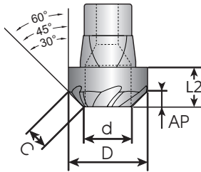
7 flutes D: 13mm
